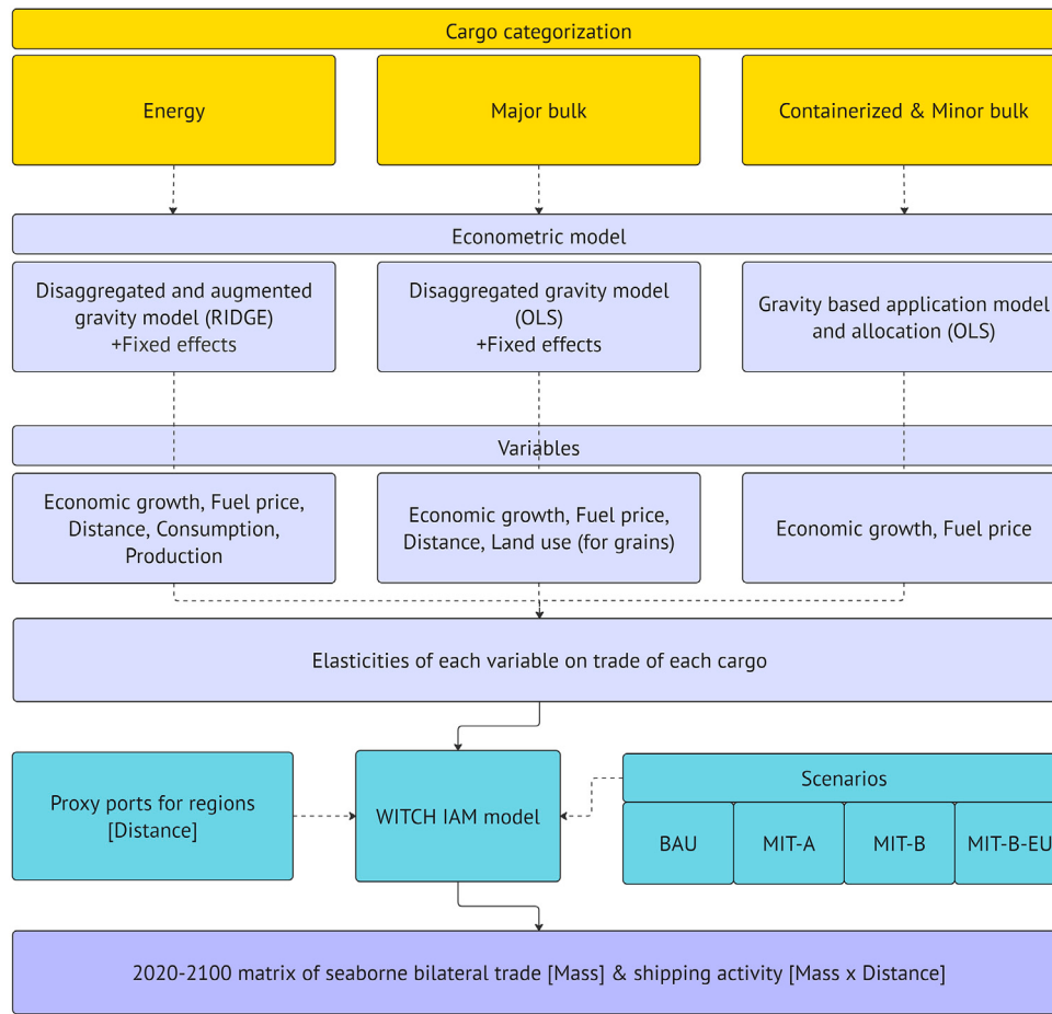
Fig. 1. Methodology framework.
